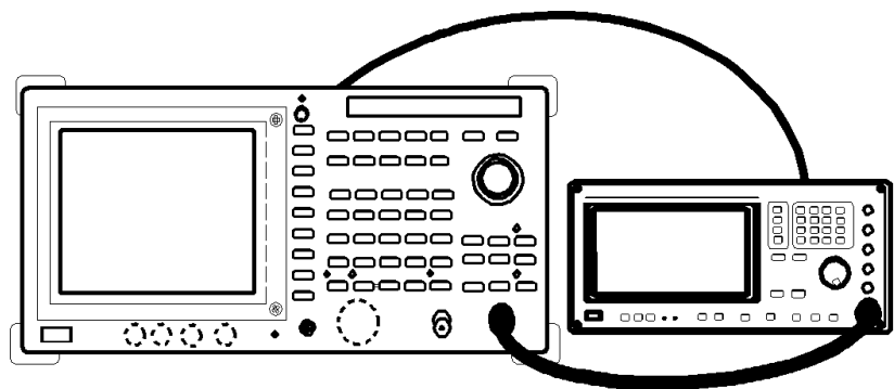
Figure 1-3 Setup for Measuring a Frequency Readout Accuracy and Frequency Counter
